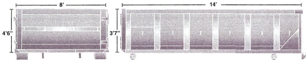
12-Yard Open - Top Container
